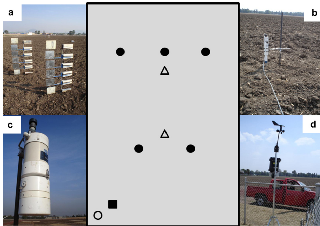
Fig. 4. Instruments layout on experimental field (center). (a) BSNE's towers (●). (b) Sensits (Δ). (c) Miniviol (■). (d) Meteorological Station (○).
